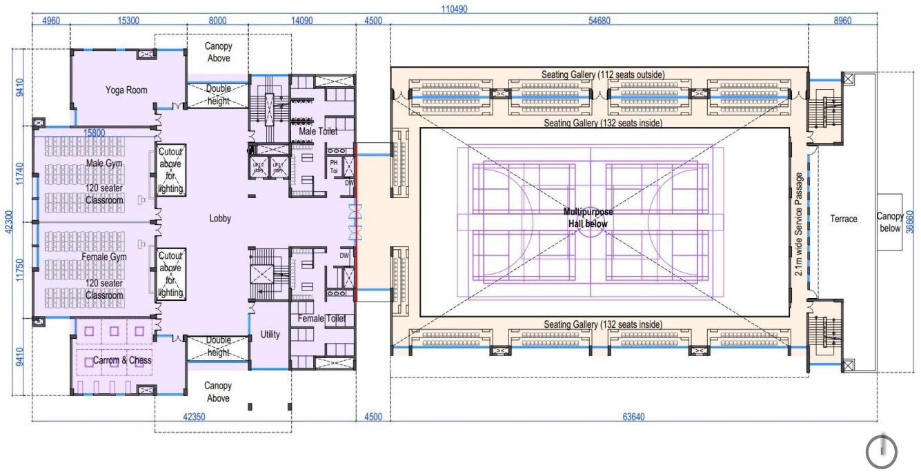
MULTIPURPOSE SPORTS BLOCK – FIRST FLOOR PLAN
